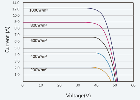
Current-Voltage & Power-Voltage Curves (540W)
