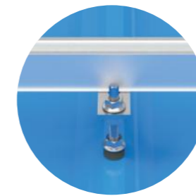
Hanger Bolt with Plate Installation
