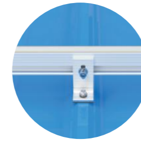
L Feet Installation
