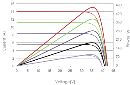
Current-Voltage & Power-Voltage Curves (415W)
