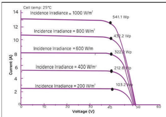
I-V Curve of 540W at 25°C cell temp. and different Irradiance level
