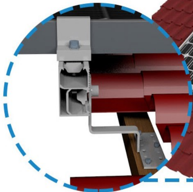
Tile roof hook
