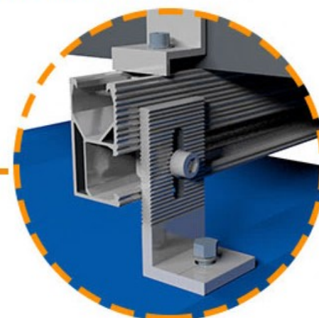
L foot
