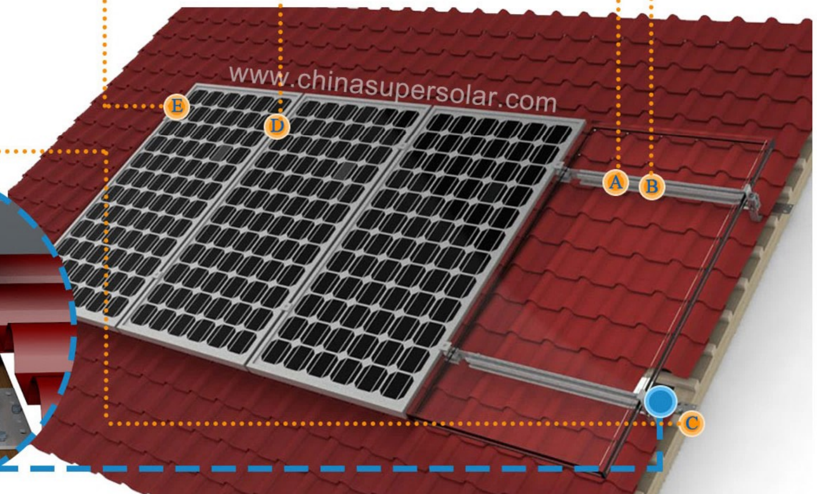
Mid clamp
