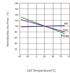
Power voltage current curve at different temperature
