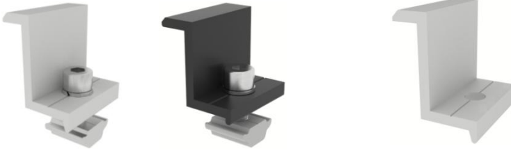
MG-AGM-EC-K-F End Clamp Kit F=25/30/32/35/40/45/46/50 mm
