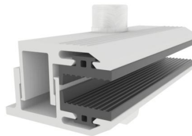
MG-TF-ECK-L80 Thin Film End Clamp Kit, 80 mm MG-TF-ECK-L120 Thin Film End Clamp Kit, 120 mm
