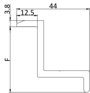
MG-AGM-EC-C-F25/30/32/35/40/45/50 End Clamp
