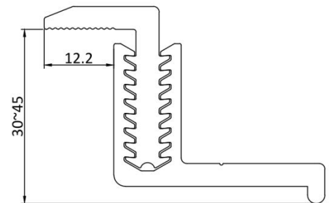
MG-TF-ECK-L80 Thin Film End Clamp Kit, 80 mm MG-TF-ECK-L120 Thin Film End Clamp Kit, 120 mm
