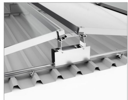
Middle support
