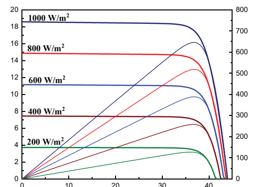
Current - Voltage & Power - Voltage Curve (CWT645-120TN12)
