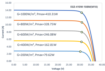
IV-Curves Irradiance
