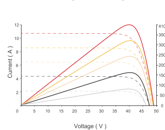
Current - Voltage & Power - Voltage Curve(415W)
