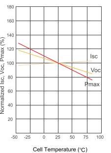
Cell Temperature Curve of I sc , V oc , P max
