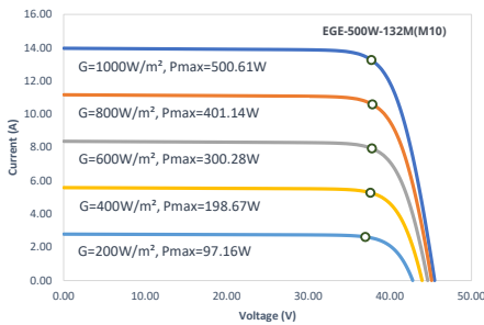
IV-Curves Irradiance
