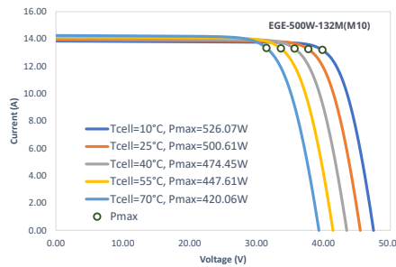
IV-Curves Temperature
