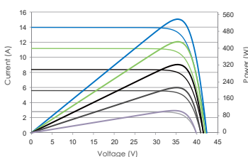
LP182*210-M-54-NH-500W
