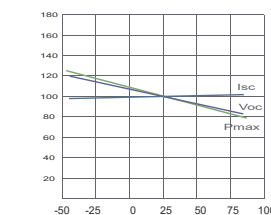
LP182*210-M-54-NH-500W
