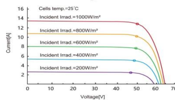
Current-Voltage Curve
