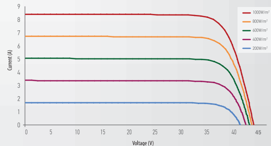
I-V Curve
