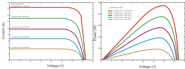
Current-Voltage & Power-Voltage Curves (SKT470M12-96D3)
