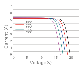
Current Voltage Curve CBG-100M/32
