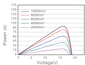
Power Voltage Curve CBG-100M/32
