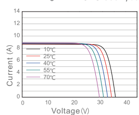
Current Voltage Curve CBG-300M/60
