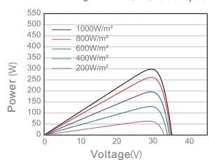
Power Voltage Curve CBG-300M/60
