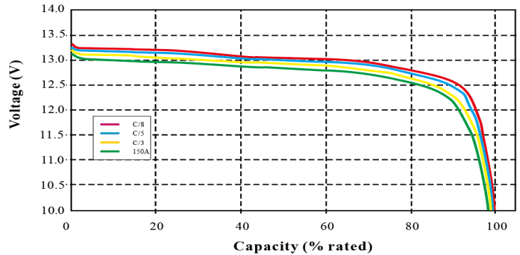
Discharge Voltage Profiles at Various Rates @25°C Ambient Temperature
