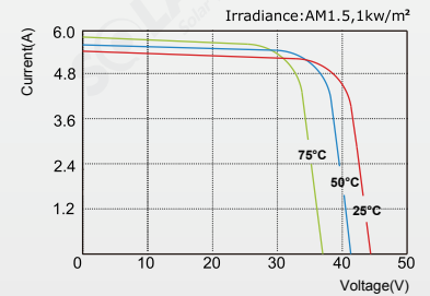
SLP190-24U I-V Curves
