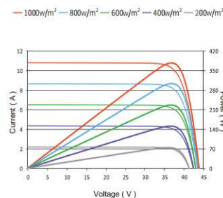
Current-Voltage & Power-Voltage Curves (355W)
