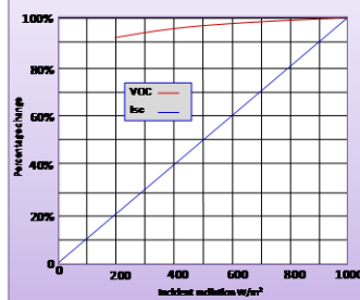
Light-Level Performance for Isc and Voc
