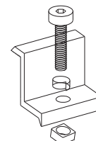
Ends Clamps tipo "Z"
