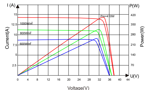
Current-Voltage&Power-Voltage Curve(410W)
