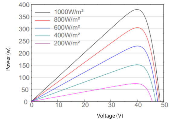
SPE 380 Power-Voltage Graph
