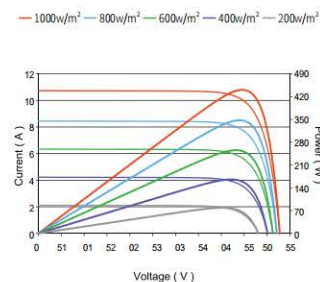
Current-Voltage & Power-Voltage Curves (450W)
