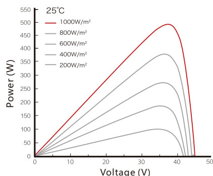
Power curve under different irradiance OLV-495-66M-HEAH
