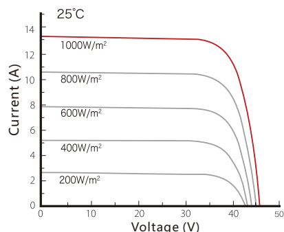
I-V Curves at Different Irradiances OLV-495-66M-HEAH
