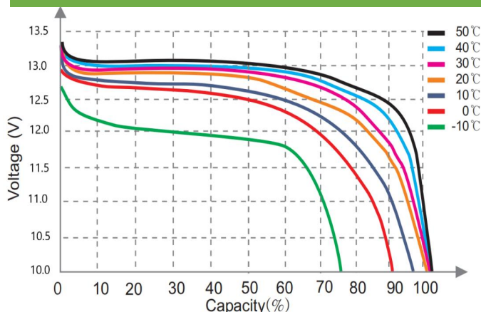
Discharge voltage curve at Different temperature
