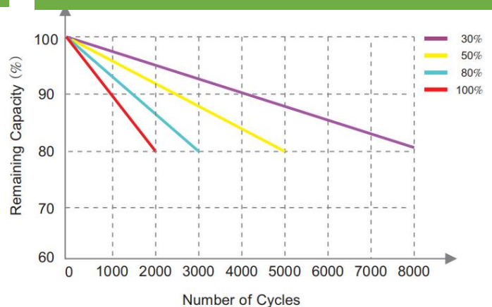
Cycle life at different DOD
