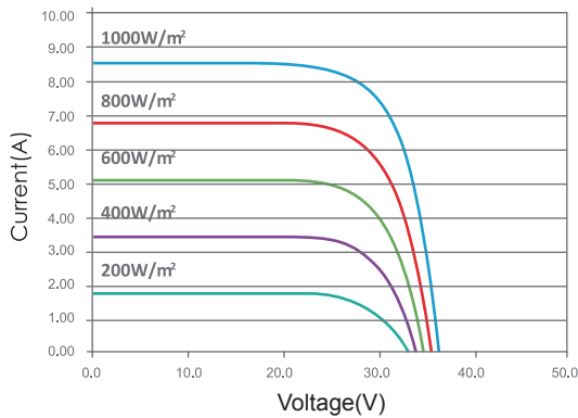
I-V Curves of PV Module SL6P60-240W (Cell Temp. 25 °C)
