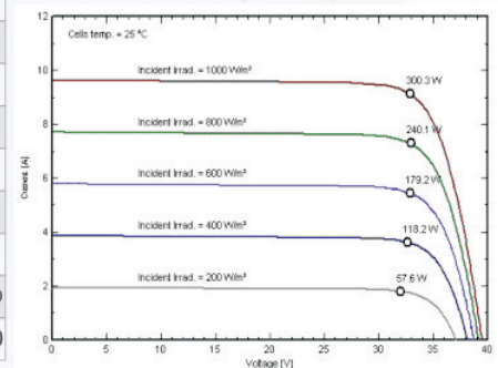
IV Curves for 300 Wp Monocrystalline Module
