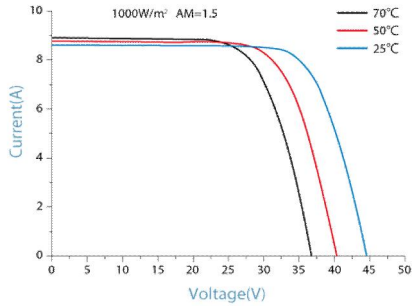
IV-CURVES of PV module RD320P6
