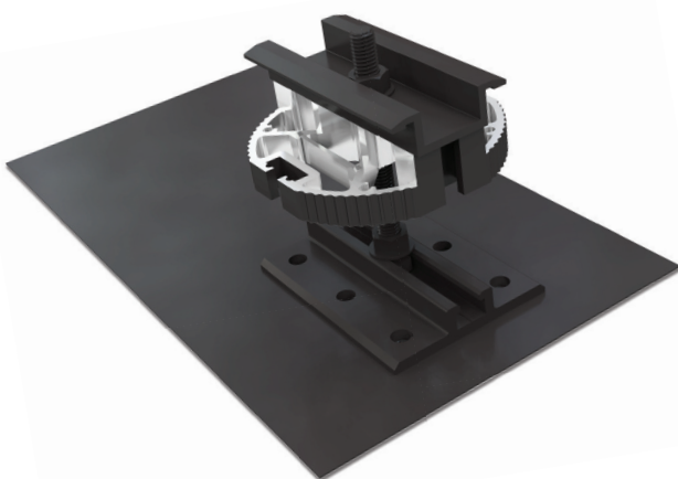
Flashing option shown – mounting screws included
