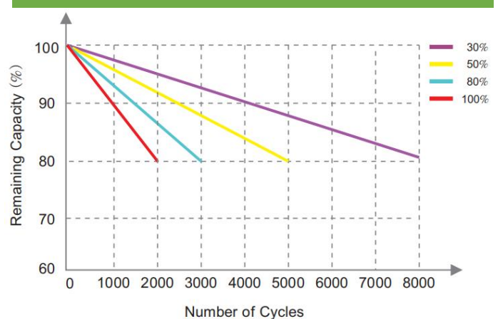
Cycle life at different DOD
