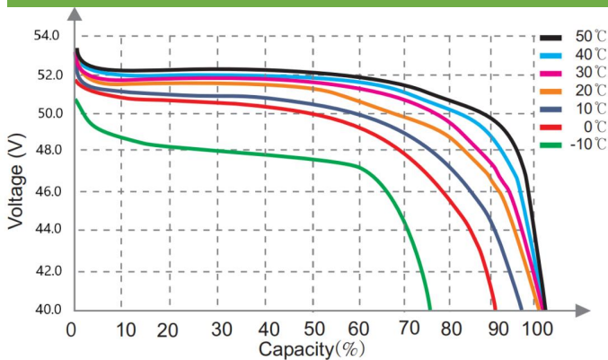
Discharge voltage curve at Different temperature
