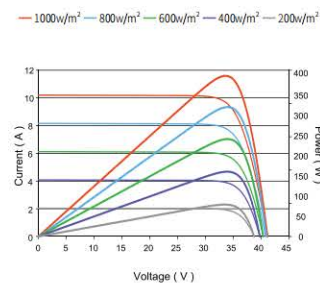
Current-Voltage & Power-Voltage Curves (390W)
