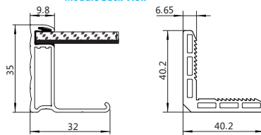
Section View
