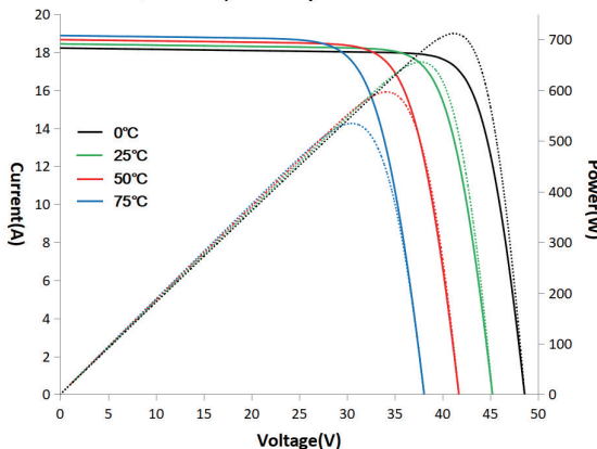
Irradiance: AM1.5, 1000W/m²
