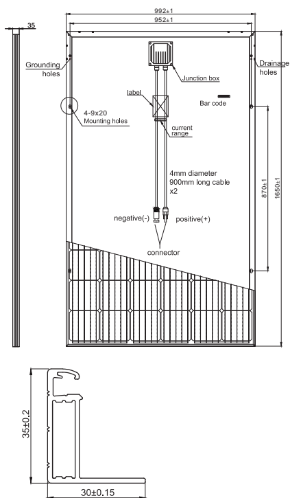
Dimension of PV Modules Unit: mm
