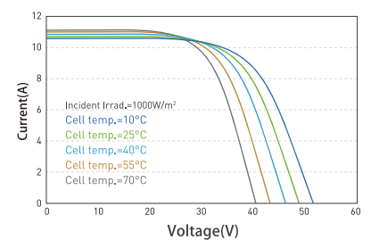
不同温度下电流电压曲线 (380W) Current voltage curve at different temperatures (380W)
