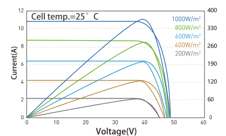
不同辐照度下电流电压曲线/功率电压曲线 (380W) Current voltage curve / power voltage curve under different irradiance (380W)
