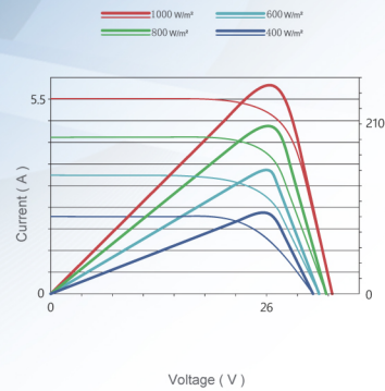
Current-Voltage & Power-Voltage Curves(210W)
