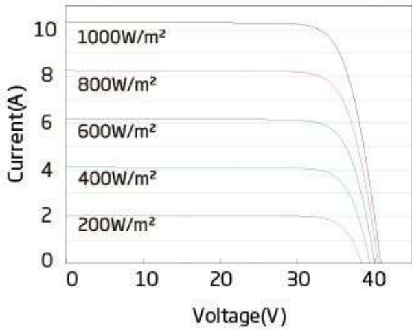
I-V CURVES OF PV MODULE(320W)
