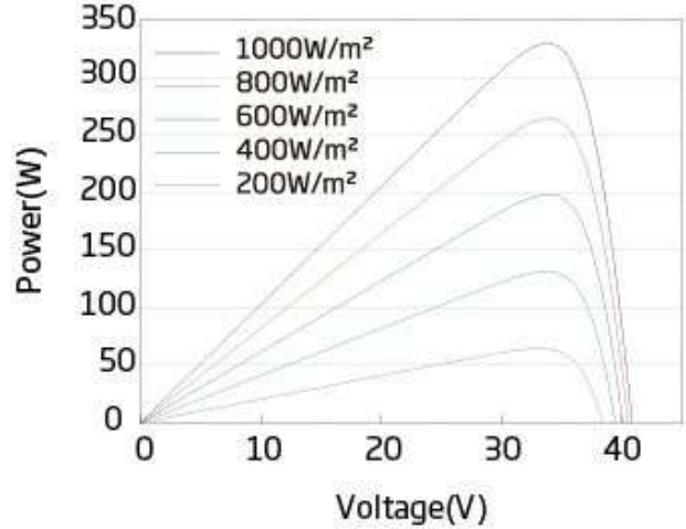
P-V CURVES OF PV MODULE(320W)
