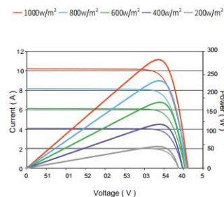
Current-Voltage & Power-Voltage Curves (290W)
