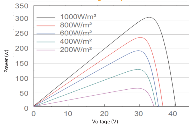
SPE 310 Power-Voltage Graph
