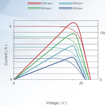
Current-Voltage & Power-Voltage Curves(170W)
