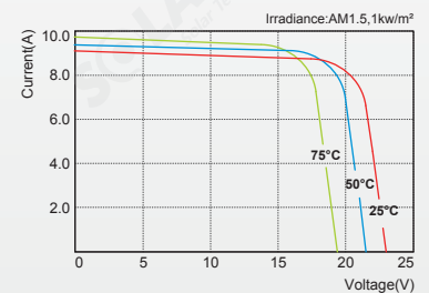
SLP160-12U I-V Curves
