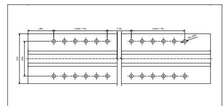
Pre-drilled holes
