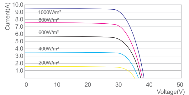
IV Curve
