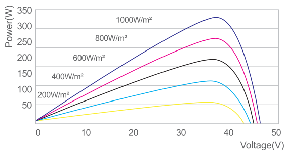
PV Curve
