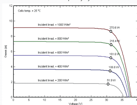
IV Curves for 270 Wp Polycrystalline Module
