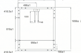
Drawing of 260Wp - 275Wp Module
