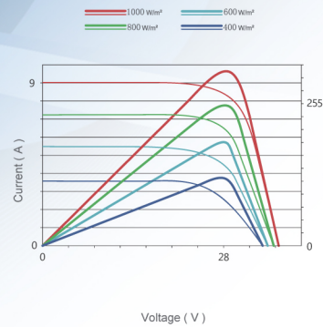
Current-Voltage & Power-Voltage Curves(255W)
