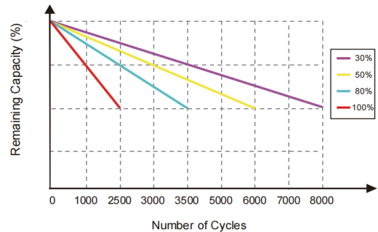
CYCLE LIFE vs. DEPTH OF DISCHARGE(DOD)
